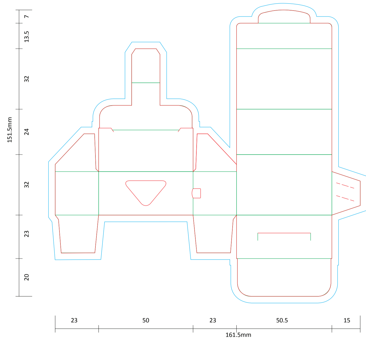
PAPER ON ROLL [1 ROLL] + FILTER TIPS [40 SHEETS] OUTSIDE ARTWORKS
