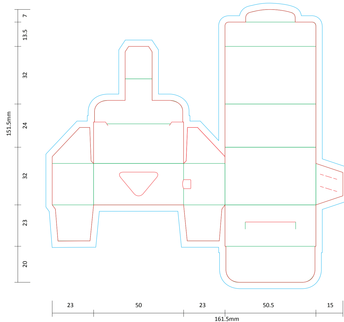
PAPER ON ROLL [1 ROLL] + FILTER TIPS [40 SHEETS] INSIDE ARTWORKS
