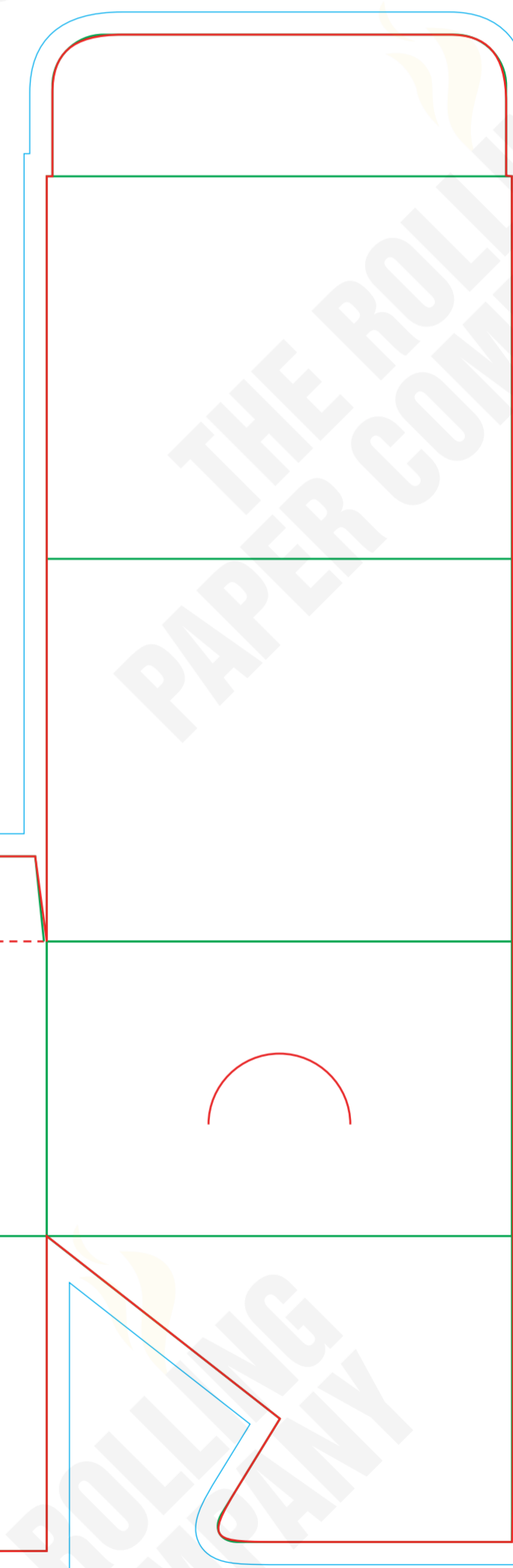
DISPLAY BOX - 25 BOOKLETS / BOX
